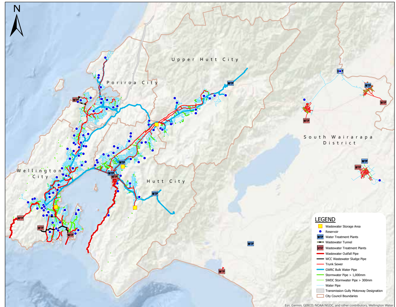
Diagram 15: Strategic three waters assets and networks (not all of the region included)
